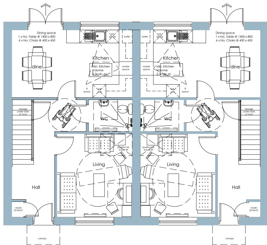
GROUND FLOOR PLAN Typical 3 Bed House Type
