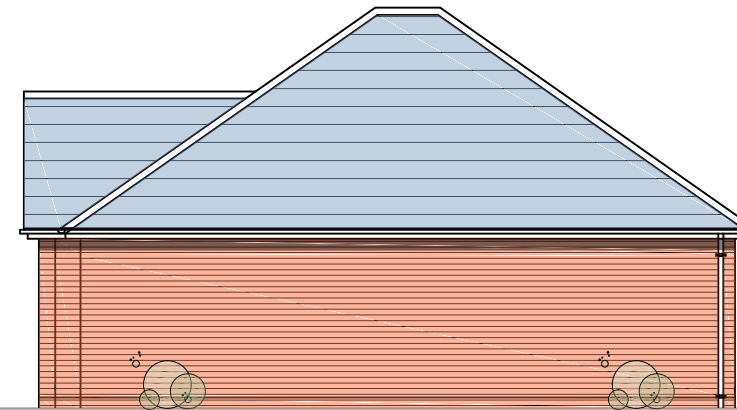
SIDE ELEVATION Typical 2 Bed Bungalow
