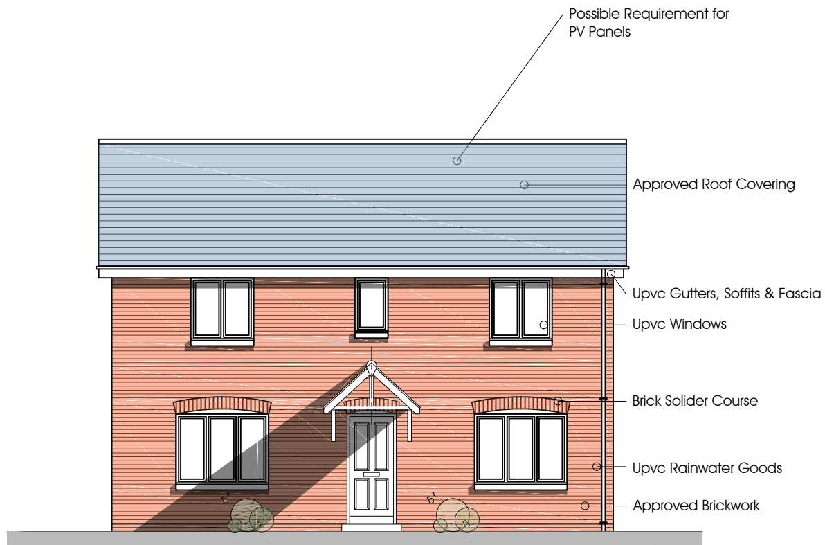
FRONT ELEVATION Typical 4 Bed House
