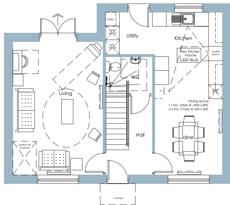
GROUND FLOOR PLAN Typical 4 Bed House Type
