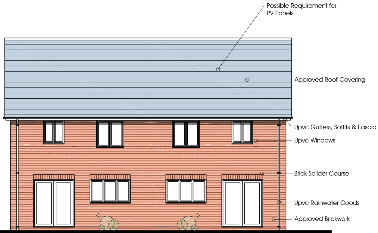
REAR ELEVATION Typical 3 Bed House
