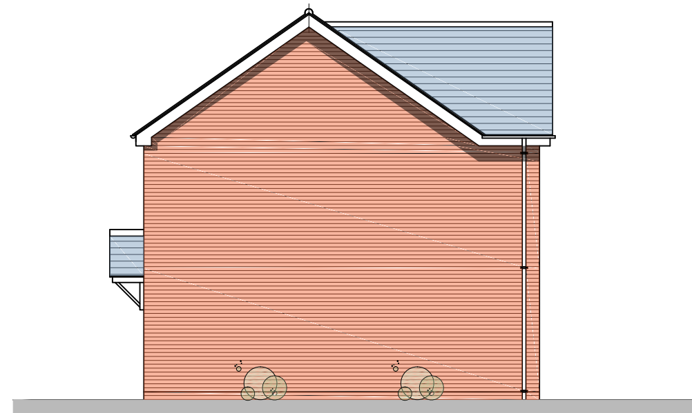
SIDE ELEVATION Typical 4 Bed House
