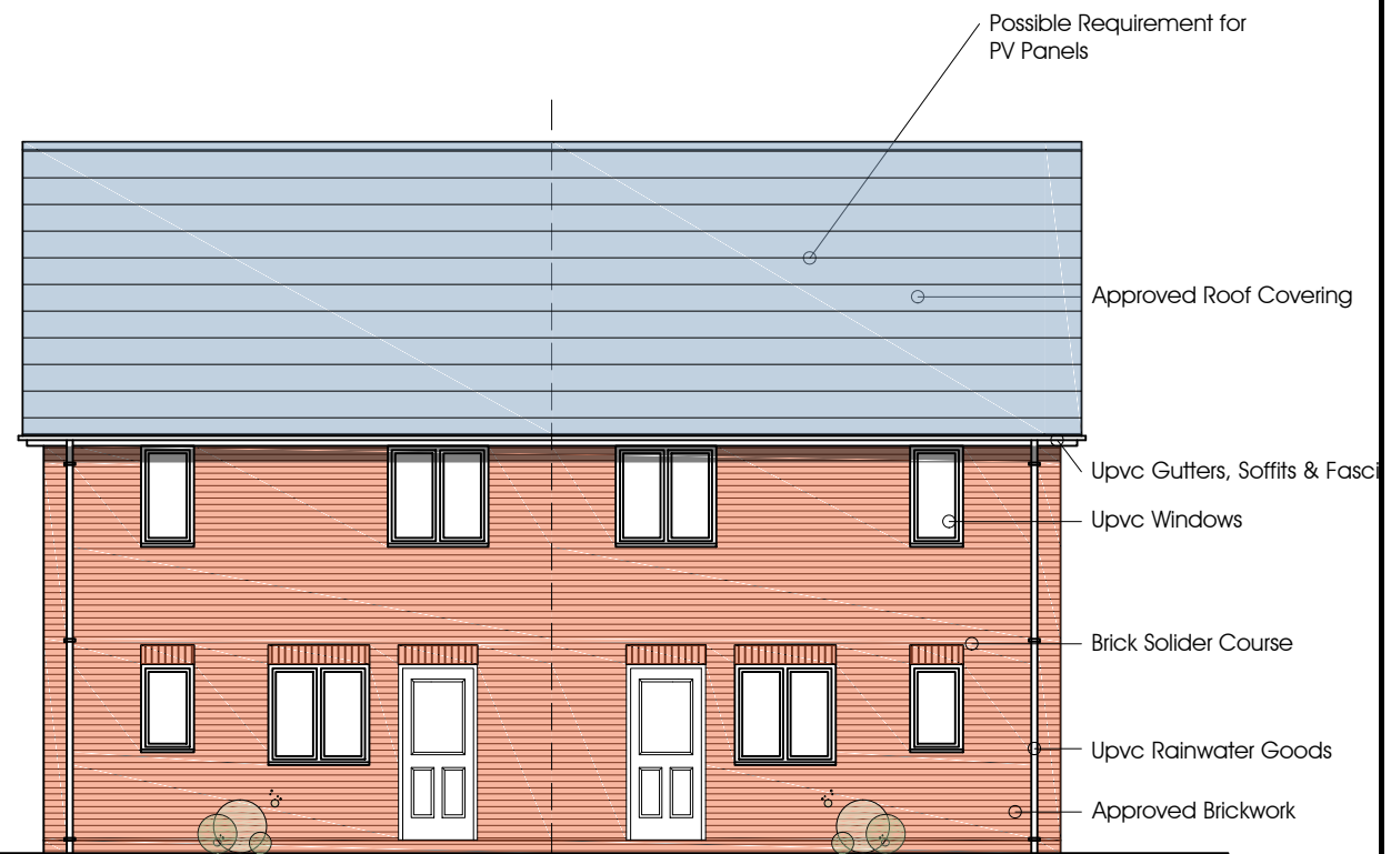
REAR ELEVATION Typical 2 Bed House
