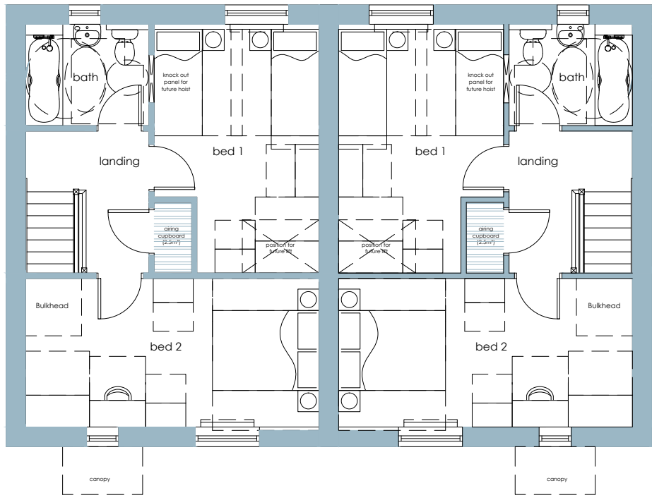
FIRST FLOOR PLAN Typical 2 Bed House
